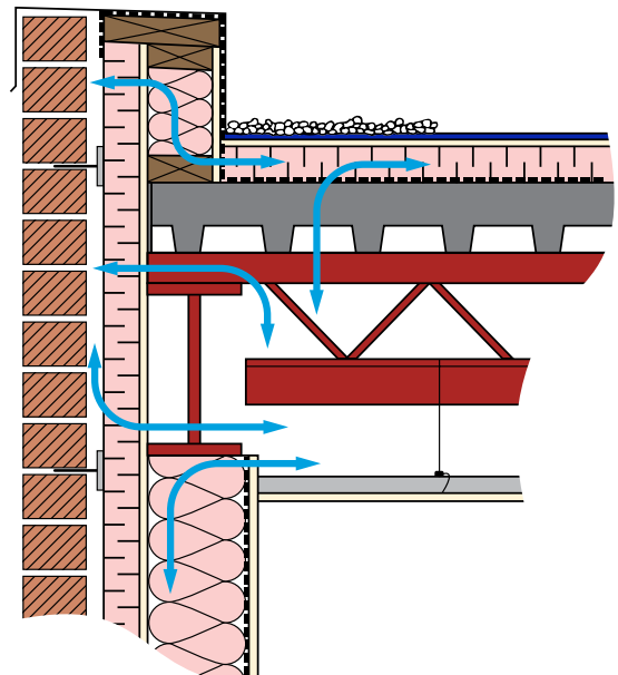
Arrows indicate air infiltration and exfiltration of the building.
